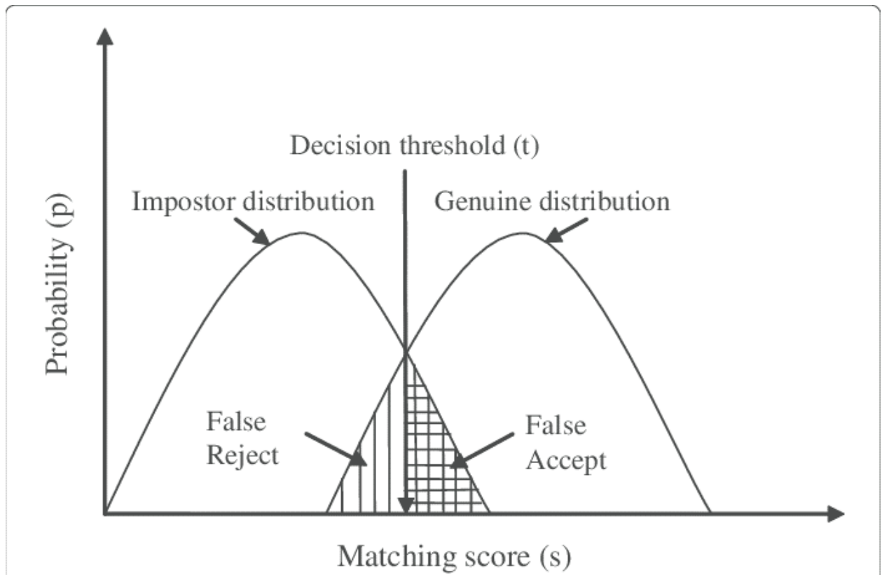
Figure 5 Impact of threshold ('matching score') on the number of False Rejects & False Accepts
